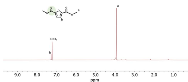
Fig. 6 1 H-NMR spectrum of CO 2 -FDME synthesized in this work.
